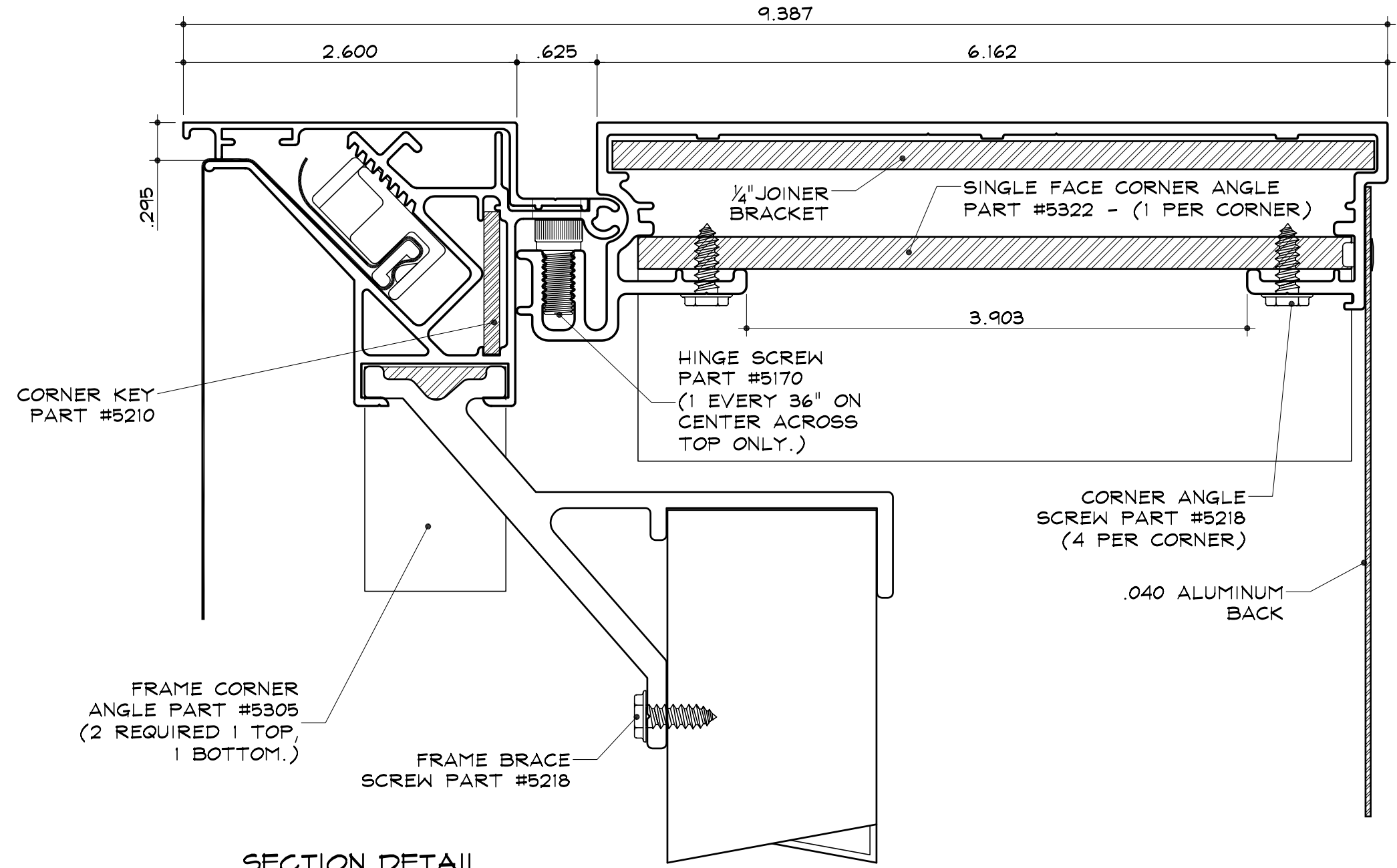
SECTION DETAIL SCALE : 1" = 1"
