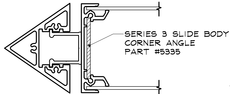
3/8" REVEAL POSITION
