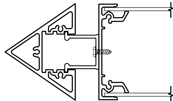
3/4" REVEAL POSITION
