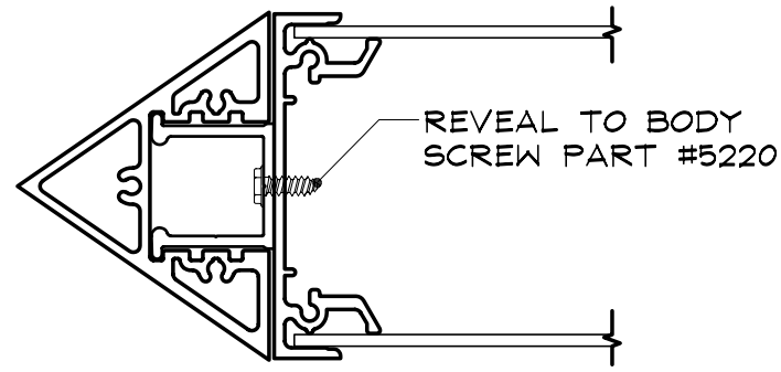
0" REVEAL POSITION
