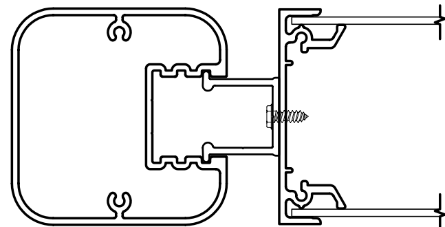
3/4" REVEAL POSITION
