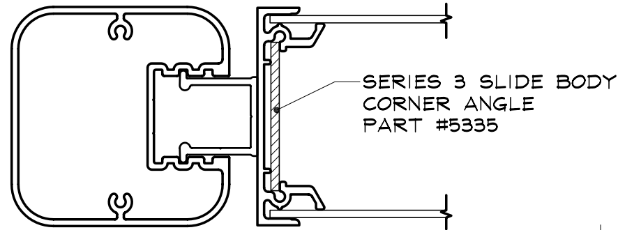
3/8" REVEAL POSITION
