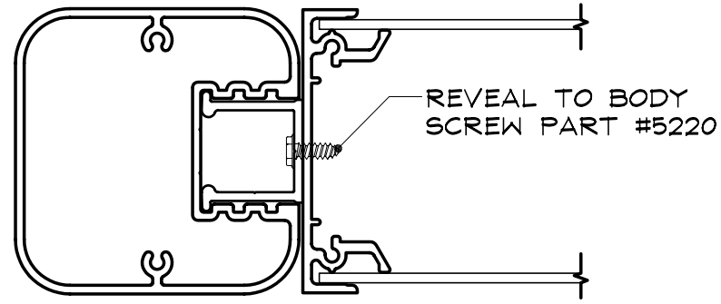
0" REVEAL POSITION
