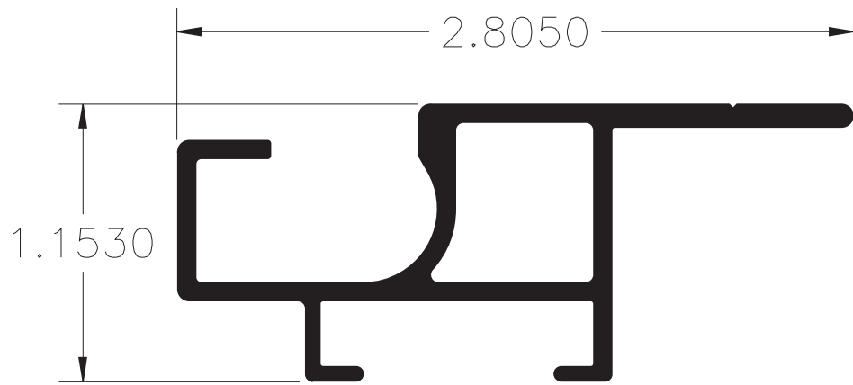
Flat Hingeable Retro Body Part #2041
