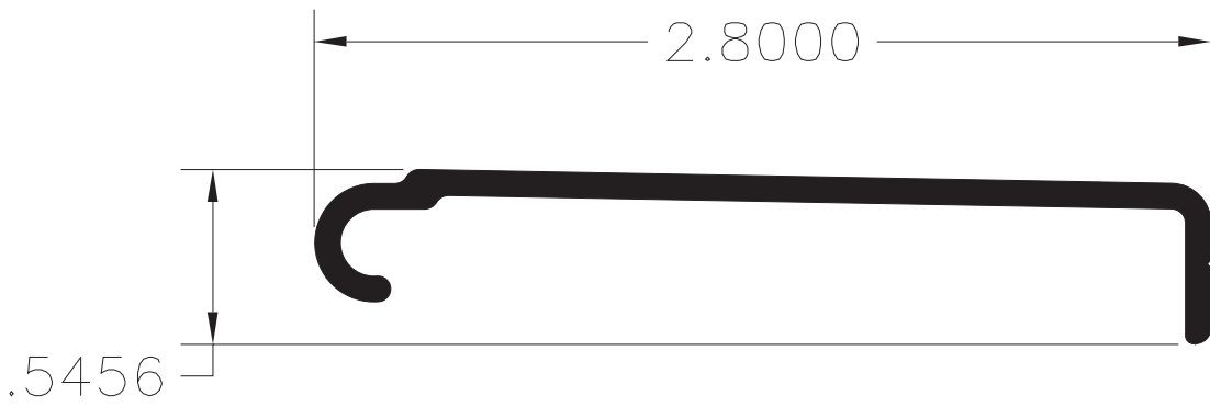
5" Narrow Channel Letter Raceway Cover Part #1976N
