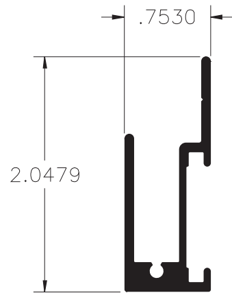
1-3/8" Wall Frame Part #1949
