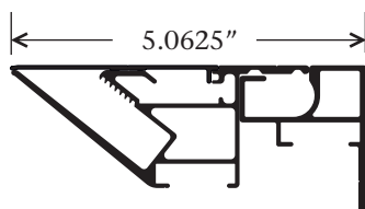
Flat Wall Mount Retro Body Part # 2042 Flat Bleed Retro Frame II Part # 2107 Flat Bleed Retro Frame Cover Part # 2121
