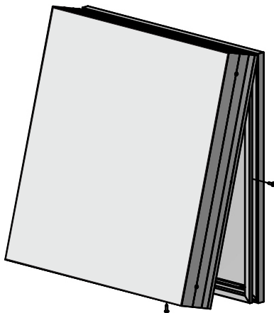
Flat Wall Mount Retro Body Part # 2042 Flat Bleed Retro Frame II Part # 2107 Flat Bleed Retro Frame Cover Part # 2121
