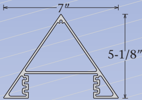
Triangular Post Part #1530
