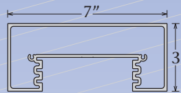
Rectangular Post Part #1510
