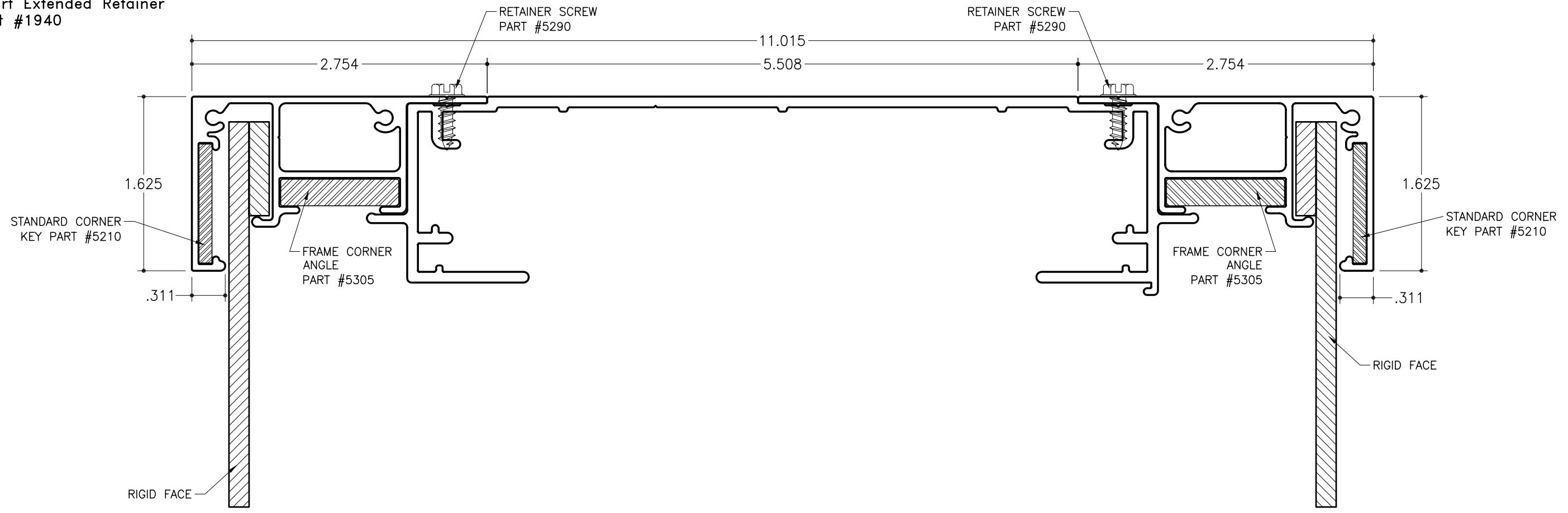
SECTION DETAIL - SIDE SCALE : 1" = 1"
