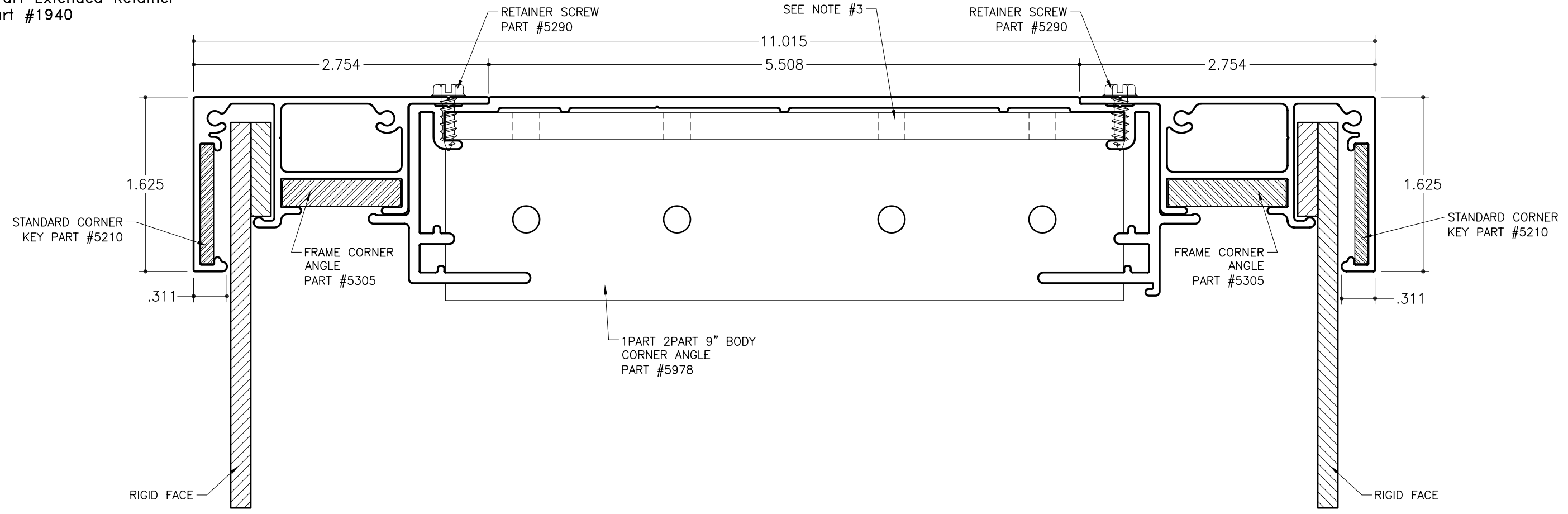
SECTION DETAIL – ADHESIVE BONDED SCALE : 1" = 1"
