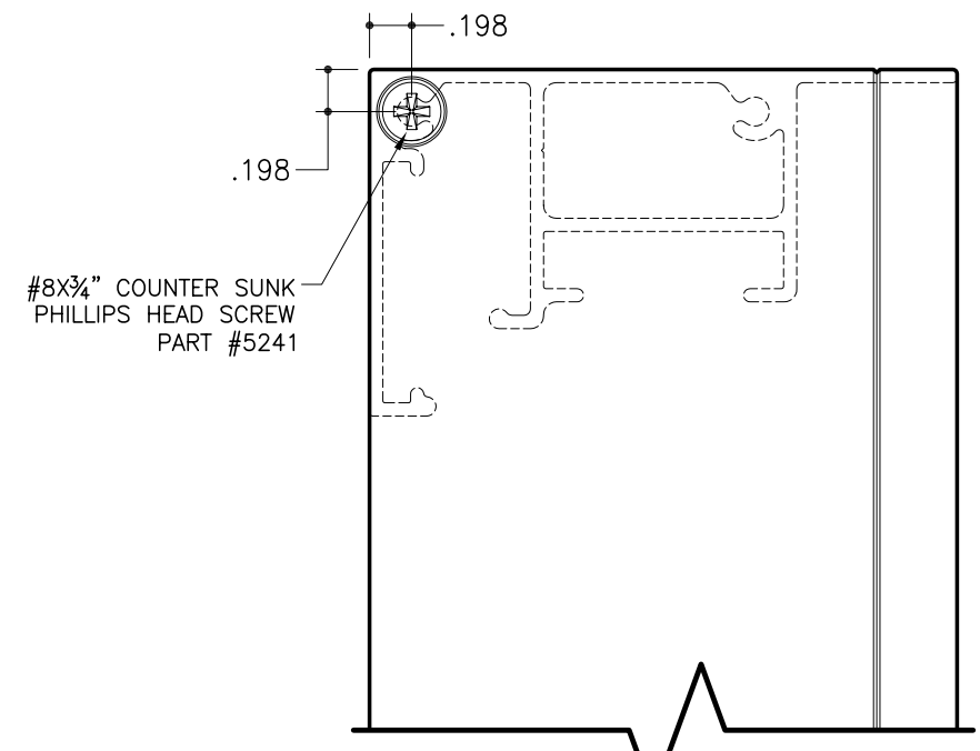
A SIDE VIEW SCALE : 1"=1"
