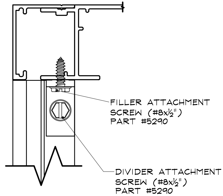
TOP VIEW SCALE : 1" = 1"
