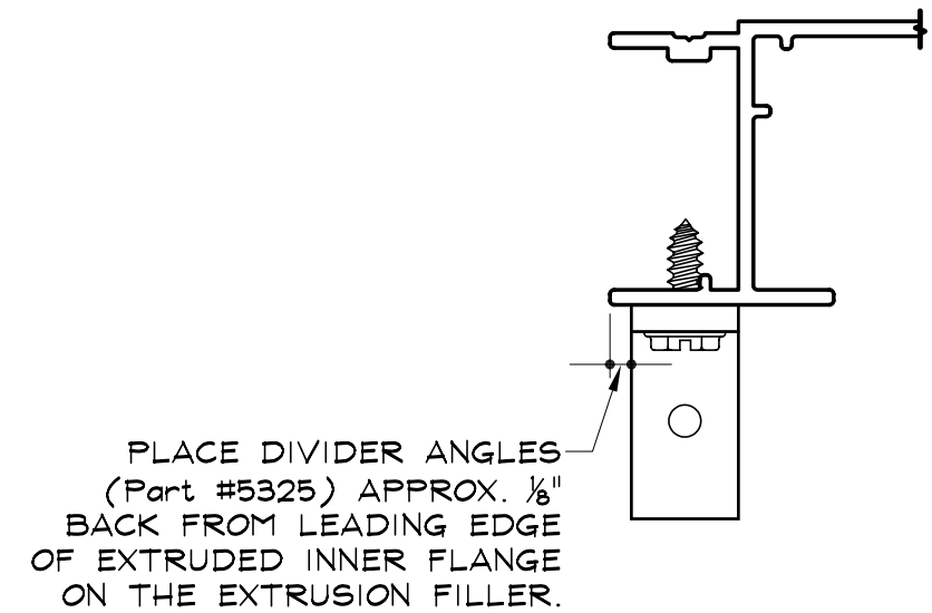
A SECTION DETAIL SCALE : 1" = 1"
