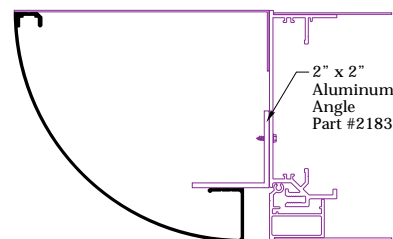
Series 7 Single Face Hinge Body and Bleed Retainer
