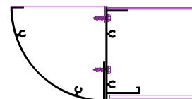
Top view of 1/4 Round End and 1/2 Slide Body
